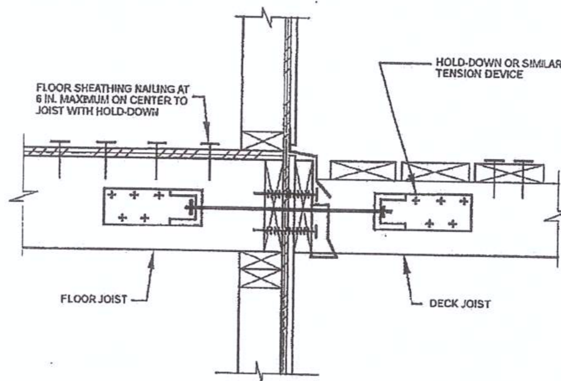
FIGURE 502.2.2.3 DECK ATTACHMENT FOR LATERAL LOADS
