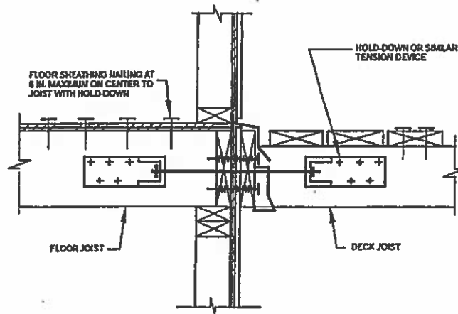
FIGURE 502.2.2.1 DECK ATTACHMENT FOR LATERAL LOADS
